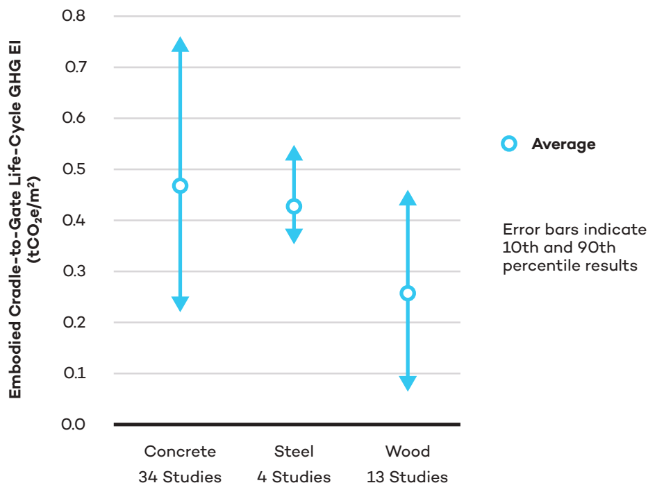
Figure 2. Embodied cradle-to-gate life-cycle GHG emission intensity of commercial buildings (tCO 2 e/m 2 )
