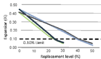
b) Mortar bars immersed for 14 days in an NaOH solution at 80°C (176°F)
