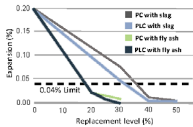
a) Concrete prisms stored for 2 years over water at 38°C (100°F)
